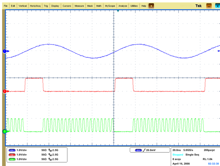
Figure 4: Output waveform from the Analog, Mkr 1, and Mkr 2 connectors
