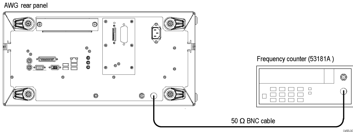
Figure 5: Equipment connection for verifying the 10 MHz reference frequency accuracy
